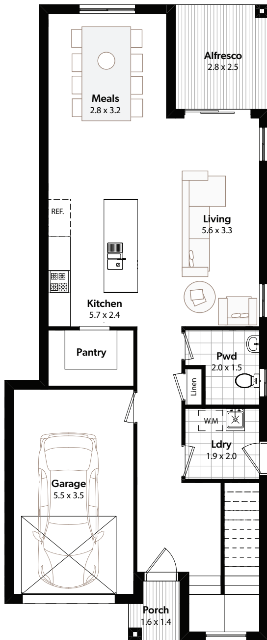
GROUND FLOOR
