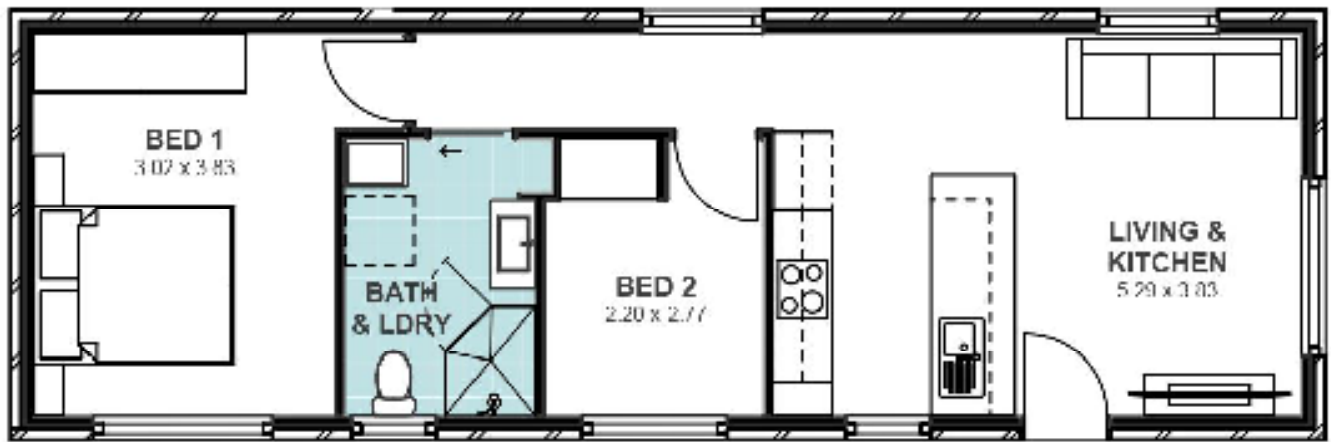
ATTACHED GRANNY FLAT
