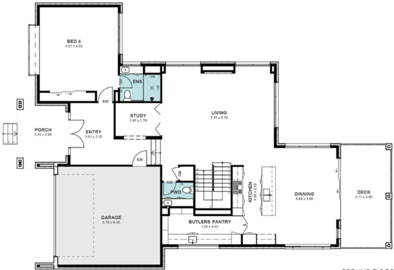
GROUND FLOOR
