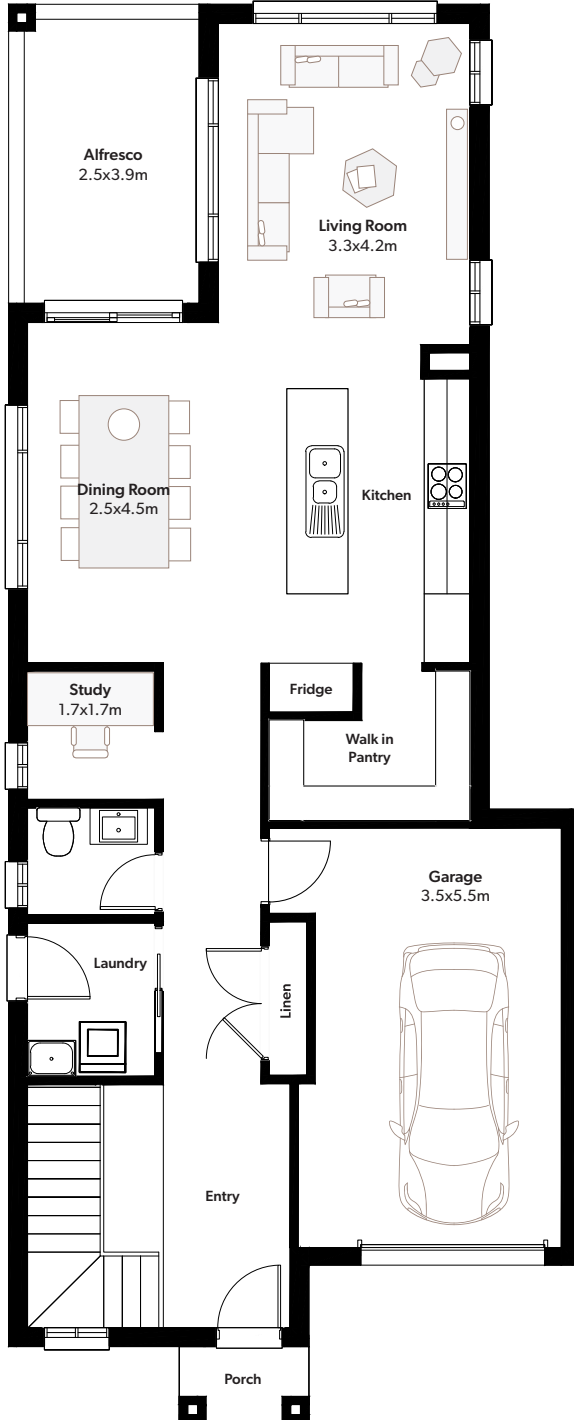
GROUND FLOOR
